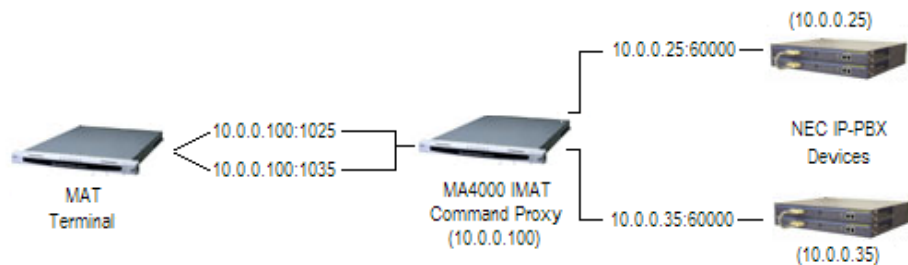
Figure 6-4 MA4000 - External Application Configuration
